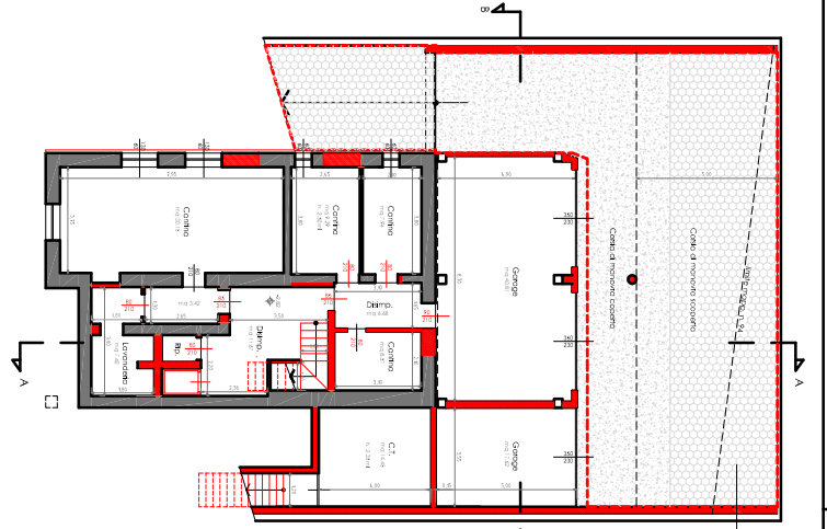
PIANO SEMINTERRATO
